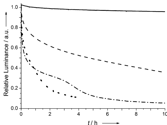
Figure 3. Plot of relative luminance against time for devices based on Ir(ppy) 3 (-----), PtON7 (.....), and PtON1 (-.-.-) with the structure ITO/HATCN/NPD/TAPC/6 % emitter:26mCPy/DPPS/LiF/Al. Also plotted are the lifetime data for the device ITO/HATCN/NPD/6%Ir(ppy) 3 :CBP/BALq/Alq/LiF/Al (—). The devices were run at a constant current of 2 \text{ mA cm}^{-2} .
